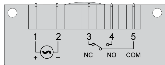
WIRING TERMINALS (polarity marked on DC models)
